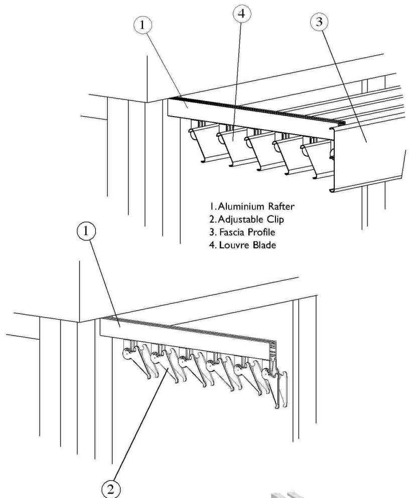
Type C100 Max Span 1.65m
