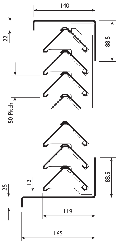
Shallow section
