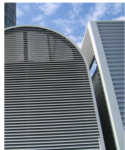
Arup Fitzrovia, London. 2UL rain defence screens for plant rooms.
