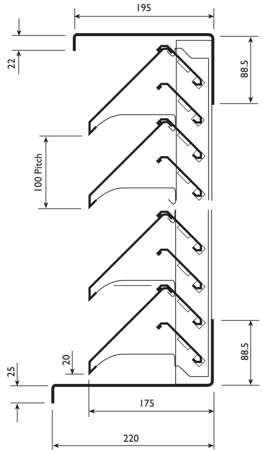
Deep section
